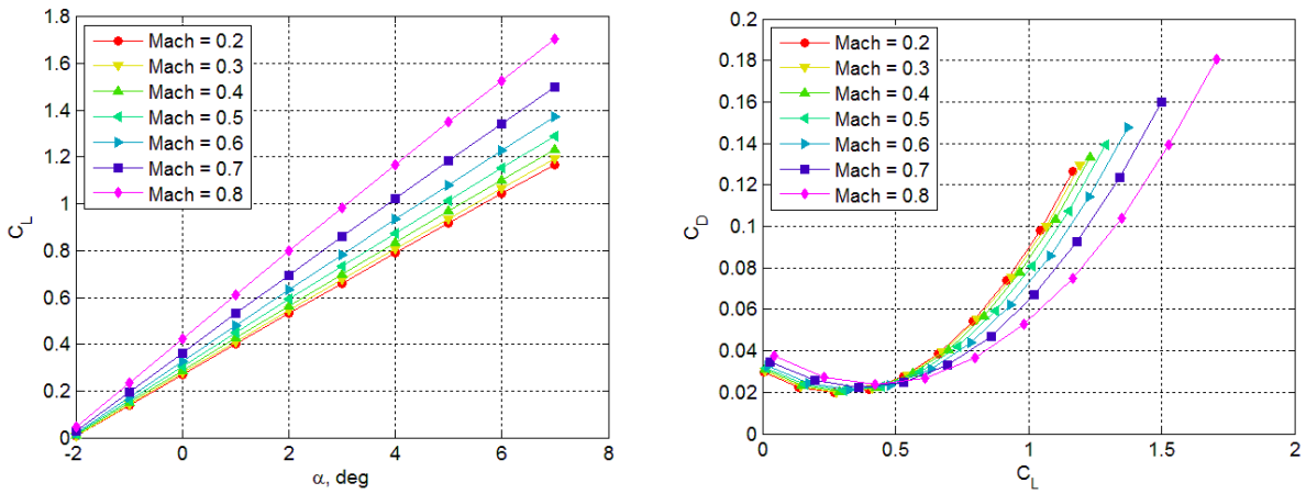
Figure 23. VORLAX Lift Curves and Drag Polars for TBW Full Configuration, Superposition Method #2
