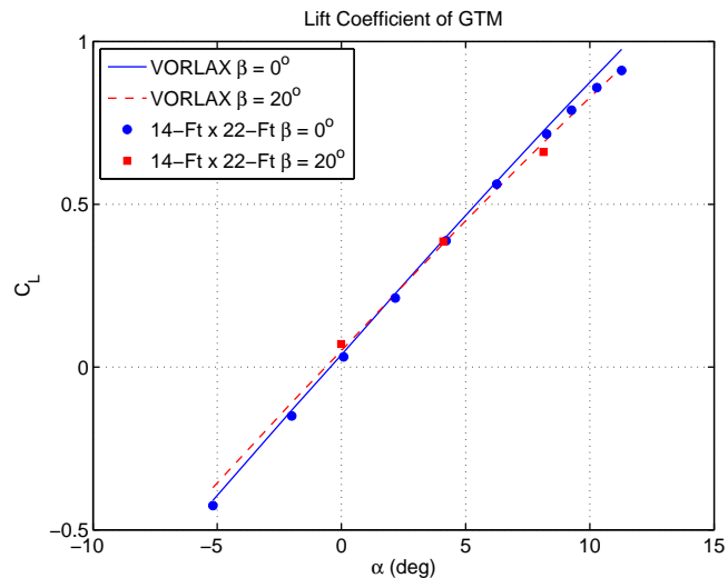
Figure 4. GTM Lift Coefficient Comparison between VORLAX and Wind Tunnel Test Data
