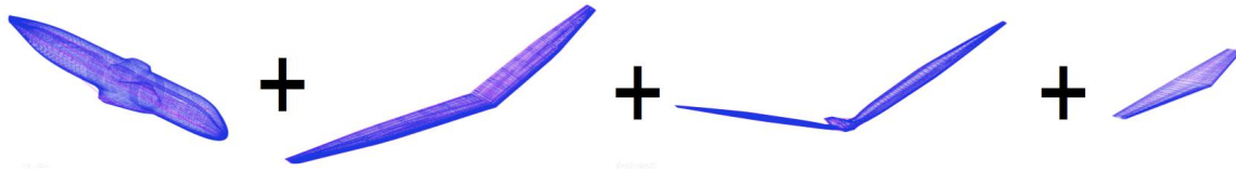
Figure 11. Aerodynamic Superposition Method 2 for TBW Model
