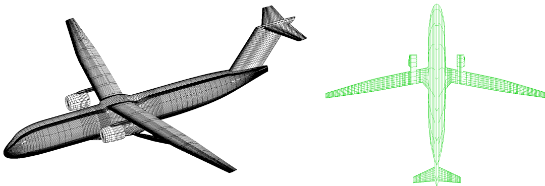
Figure 5. TBW Mesh (Left) and Vortex-Lattice Panel/Polygon Discretization (Right) in VORVIEW
