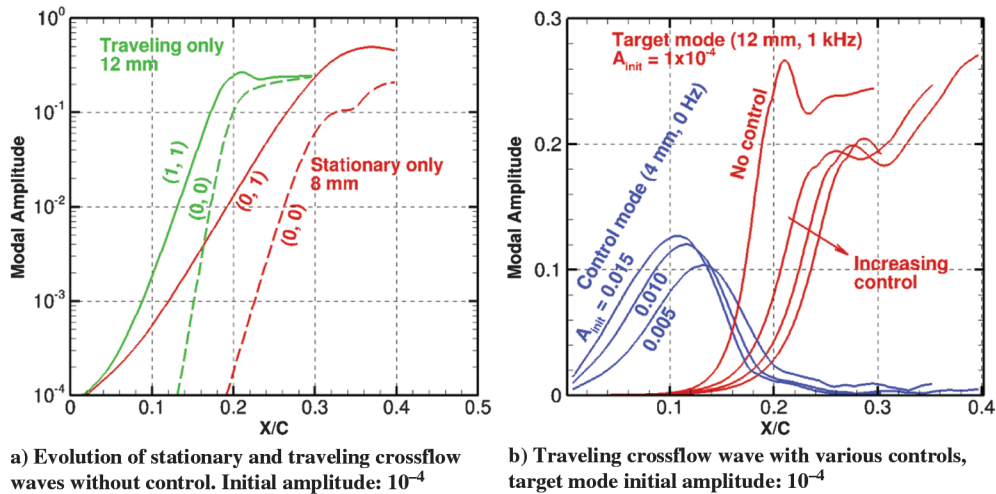
Fig. 15 Effect of control on traveling crossflow vortices.
