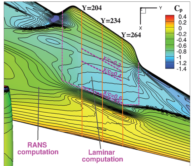
Fig. 2 Upper-surface C_p distribution computed using FUN3D.
