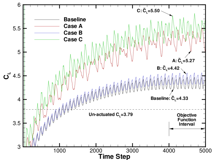
FIGURE 2. UNSTEADY LIFT PROFILES FOR THE BASELINE AND OPTIMIZED HIGH-LIFT WING CONFIGURATION. TAKEN FROM [20].
