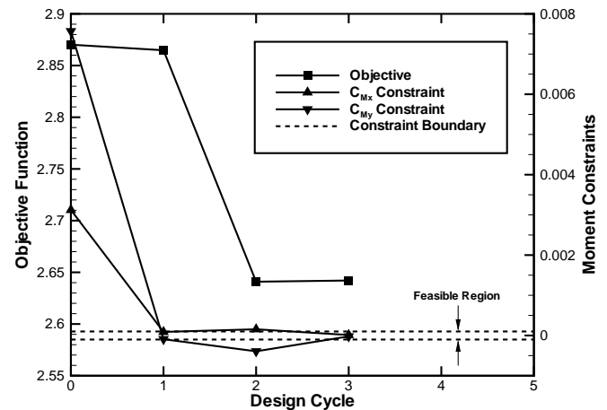
FIGURE 7. CONVERGENCE OF THE OBJECTIVE FUNCTION AND CONSTRAINTS FOR THE UH-60A CONFIGURATION. TAKEN FROM [17].
